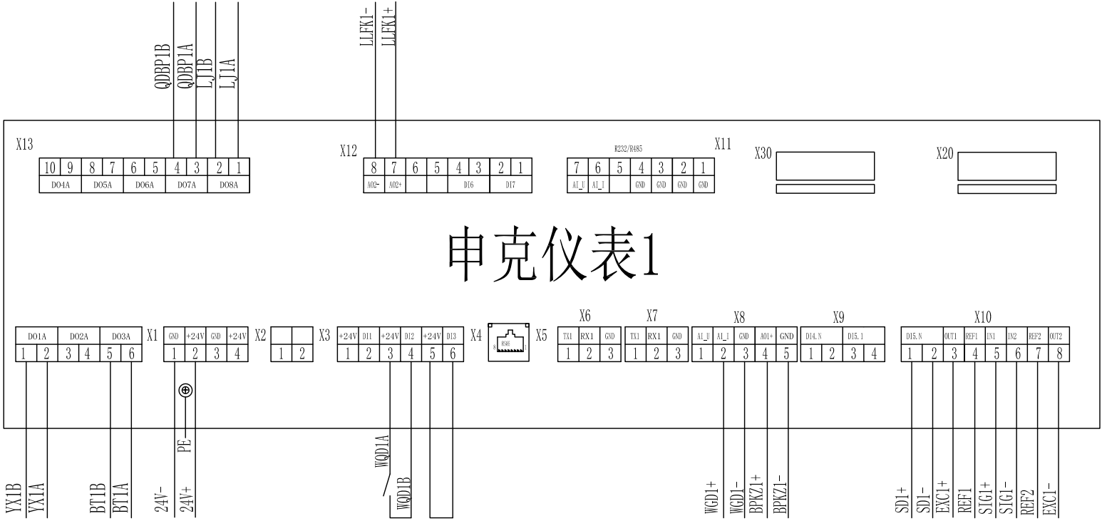
接线端子JX1
