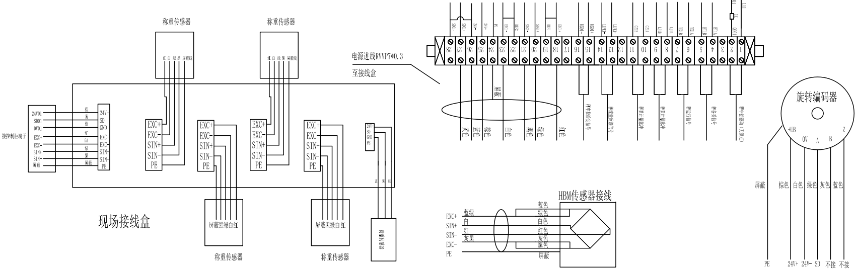
接线端子JX1
